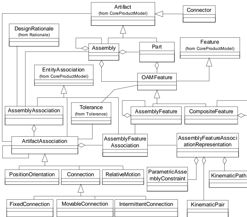
Figure 1: Class Diagram of the Open Assembly Model.
