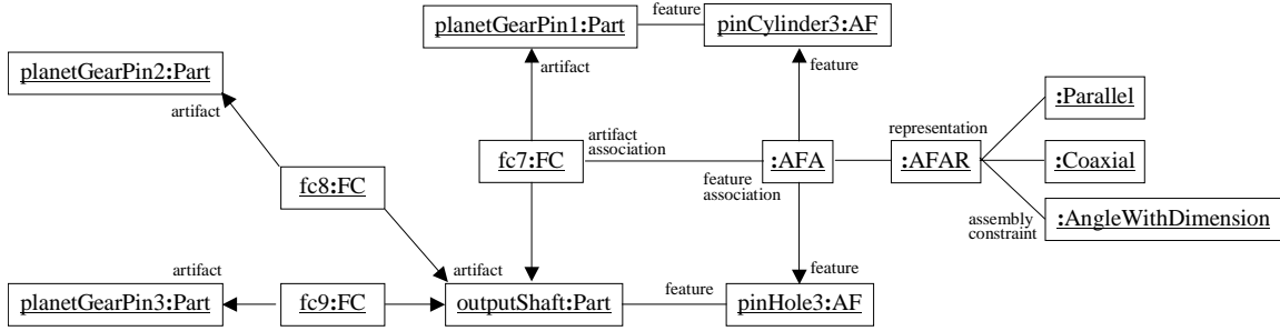
Figure 8: Instance Diagram of Planet Carrier Assembly.
