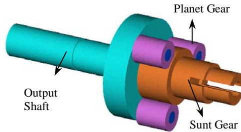
Figure 11: Planet Gear Carrier and Sun gear Assembly.
