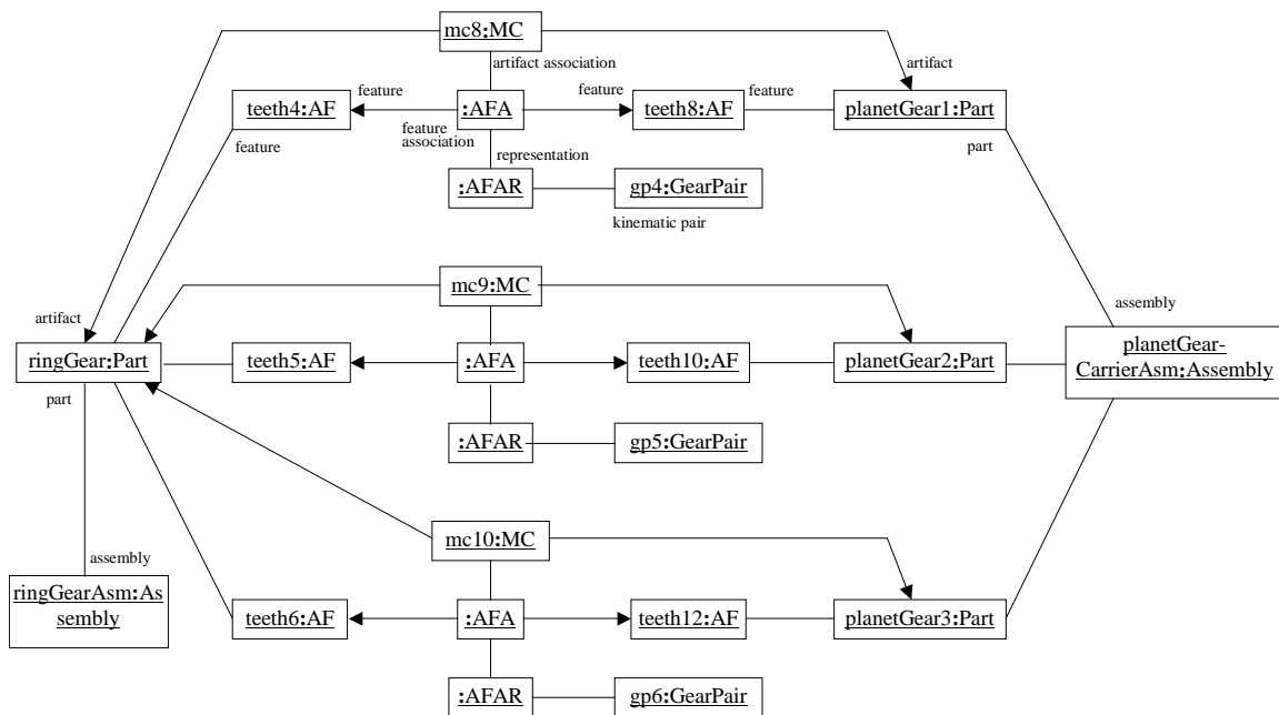
Figure 14: Instance Diagram of Planet Gear Carrier and Ring Gear Assembly.
