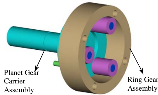
Figure 13: Planet Gear Carrier and Ring Gear Assembly.
