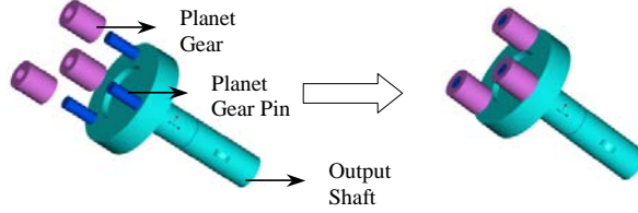
Figure 9: Planet Gear Carrier Assembly.
