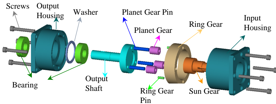
Figure 3: Exploded View of the Planetary Gear Model.
