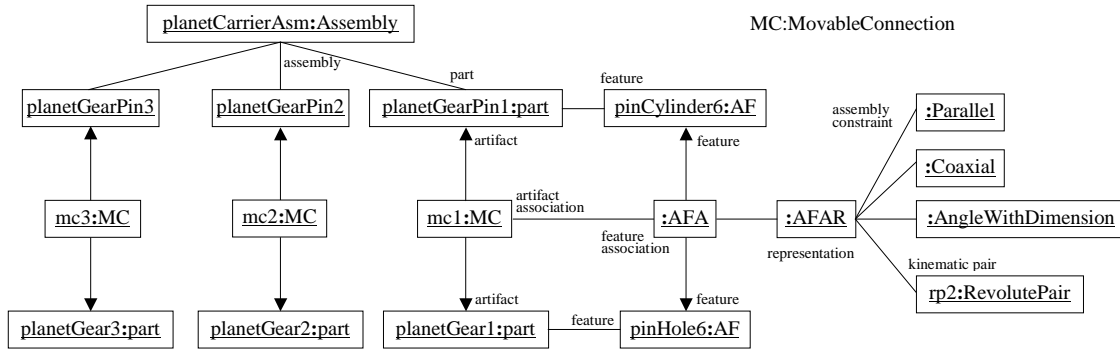
Figure 10: Instance Diagram of Planet Gear Carrier Assembly.
