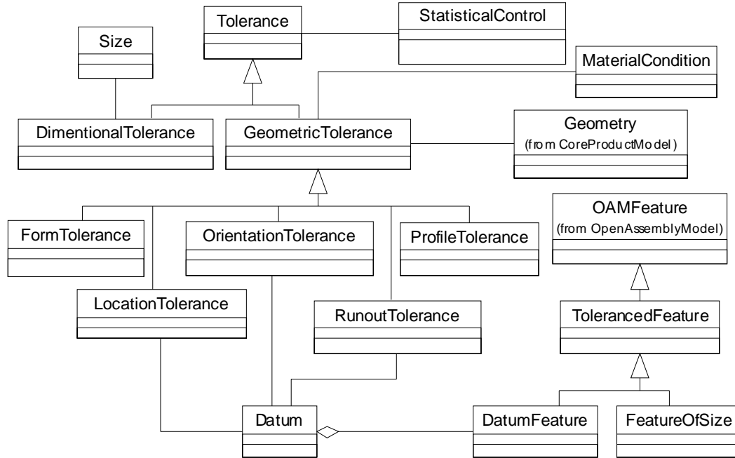
Figure 2: Tolerance Model.
