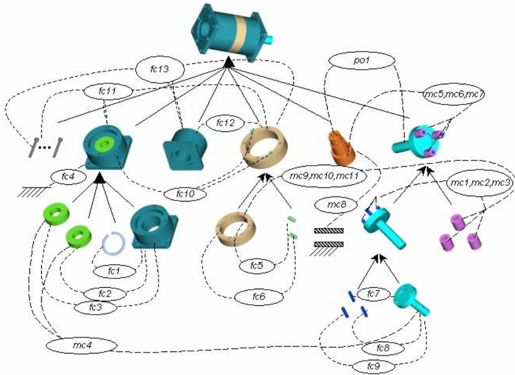
Figure 4: Artifact Associations in the Planetary Gear System.
