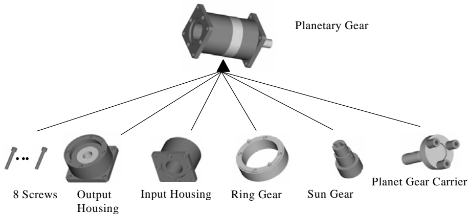
Figure 4 The Planetary Gear System
