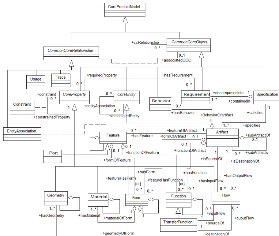
Figure 1 Class Diagram of the Core Product Model
