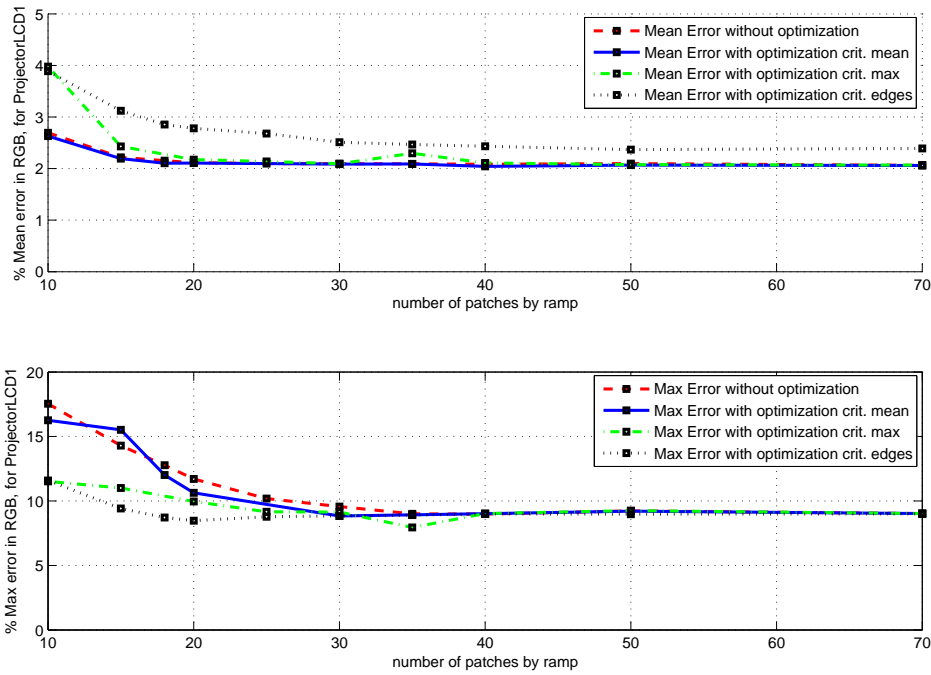
Figure 6. Algorithm performance for ProjectorLCD1, depending on the way to optimize the grid and on the number of patches used. The “edges” criterion reduces the maximum error for the same number of patches.
