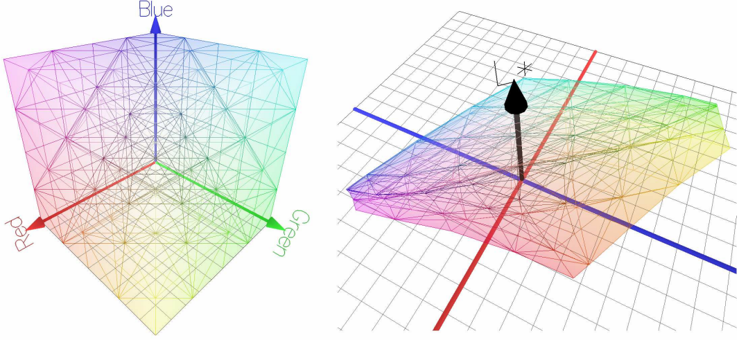
Figure 2. Tetrahedral structure based on a regular grid, N_{rgb} = 5 in RGB (left) and its transform into CIELAB (right).
