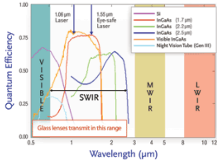
Figure 2. SWIR Wavelength [10]
